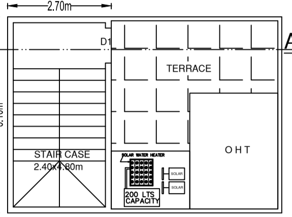
PROPOSED TERRACE FLOOR PLAN
